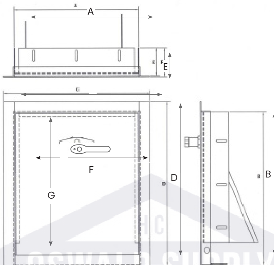
MIDLAND "STYLE" STAINLESS STEEL TRASH CHUTE DOOR DIMENSION CHART (LESS TRIM)
