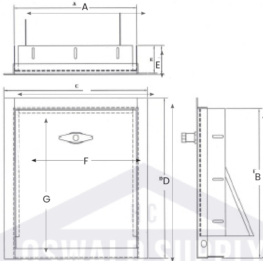
MIDLAND "STYLE" STAINLESS STEEL TRASH CHUTE DOOR DIMENSION CHART (LESS TRIM)
