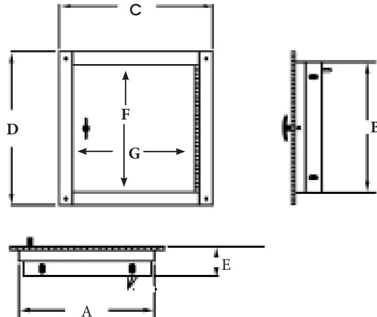
MIDLAND “STYLE” STAINLESS STEEL LINEN CHUTE DOOR DIMENSION CHART (WITH CONNECTED TRIM – STANDARD WIDTH 2.13”)
